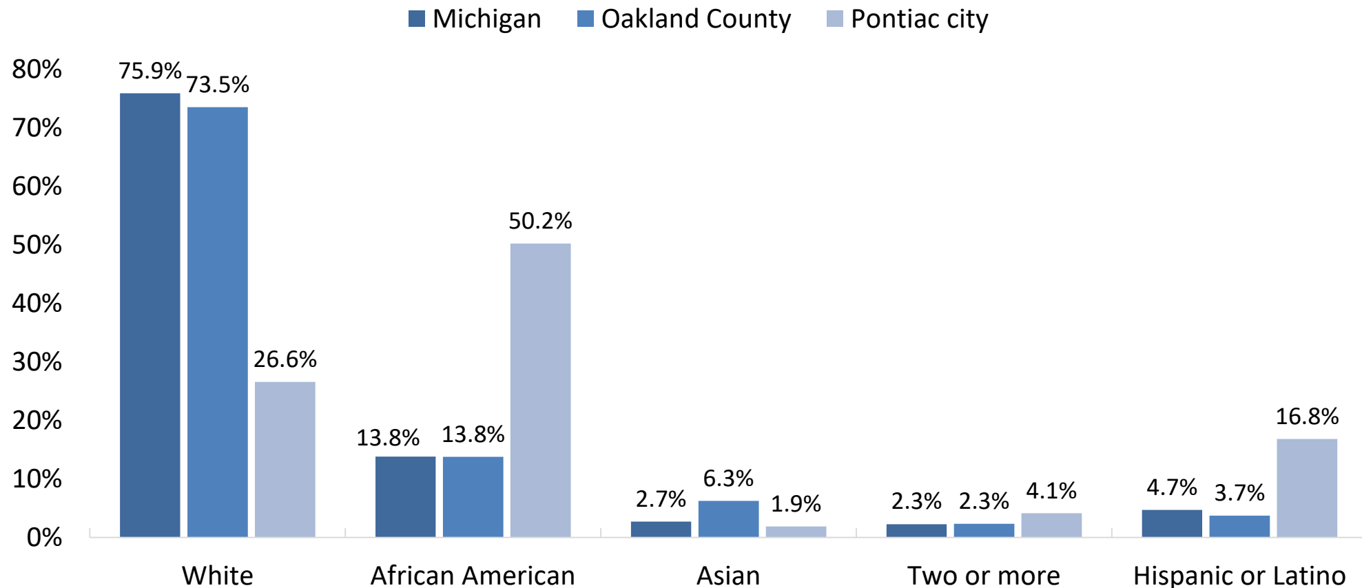
Figure 4: Racial/Ethnic Breakdown, 2011-2015
